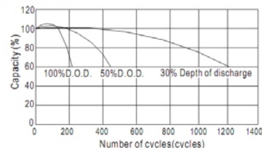
Cycle Life(25°C)
