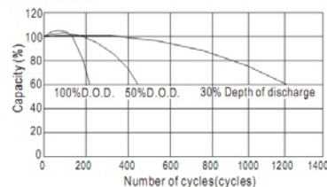
Cycle Life(25°C)
